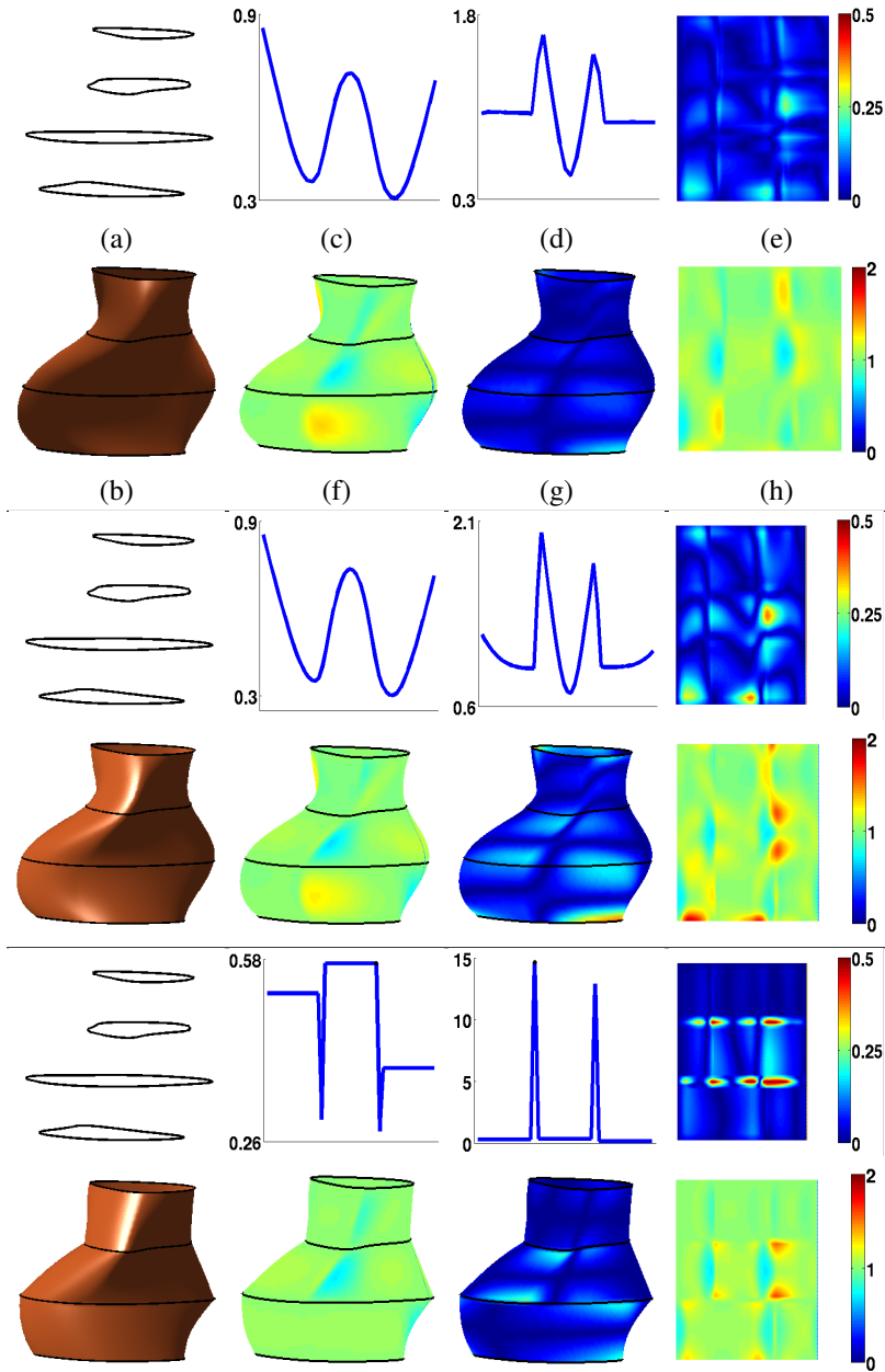
Figure 1: a: original curves, b: reconstructed surface S_{MRI} , c: \|\hat{n}\| , d: \|\hat{n}\| , e: \|\nabla^2 S_{MRI}(r, \theta)\| , f: \|\nabla_r S_{MRI}(r, \theta)\| , g: \|\nabla_\theta S_{MRI}(r, \theta)\| , and h: \|\nabla S_{MRI}(r, \theta)\| . The two first rows correspond to the solution from [1], the two next to the solution from [6] and the last two to piecewise-geodesics.
